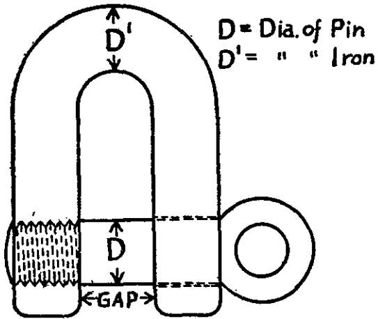
D SHACKLE.
