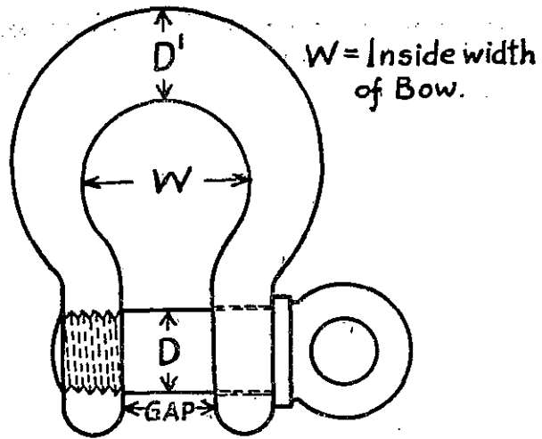
BOW SHACKLE.
